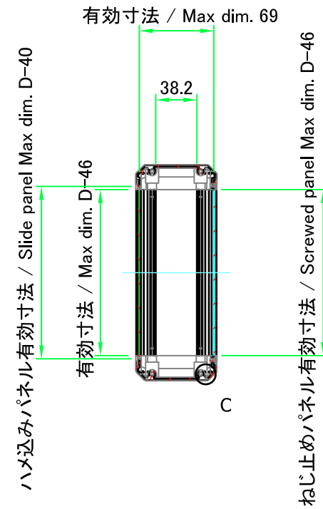
B-B (1:5)
